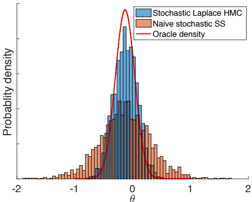
Figure 7. Naïve stochastic slice sampling vs. Stochastic Laplacian HMC.
