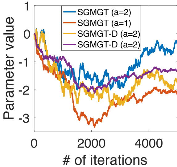
Figure 6. Traceplot for RNN experiments.
